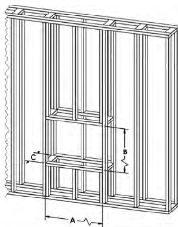
Rough Opening
