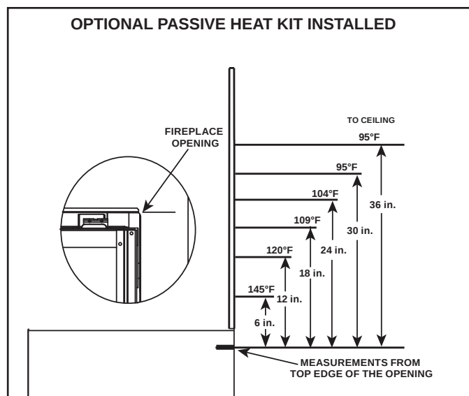
Figure 2.2 Good Faith Wall Surface Temperatures Above Appliance with Passive Heat Kit Installed
