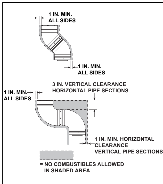
Figure 5.2 Clearances from Vent to Combustible Framing Materials
