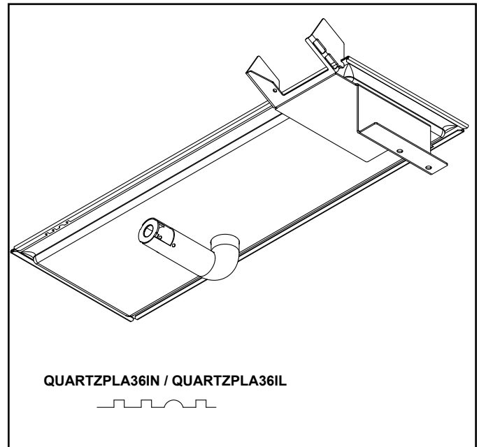
Figure 9.2 Burner Identification
